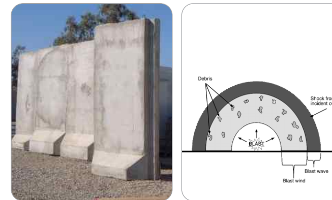
RCC- T wall and Normal RCC wall for blast protection
