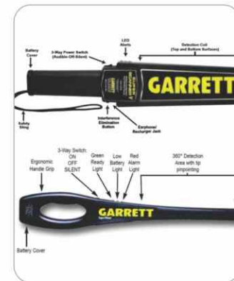
Hand Held Metal Detectors
