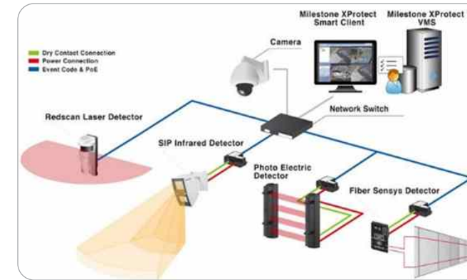
Parameter Intrusion Detection System
